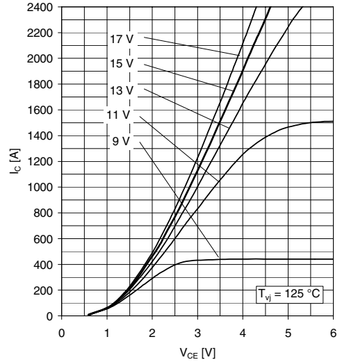
Fig. 2 Typical output characteristics, chip level
